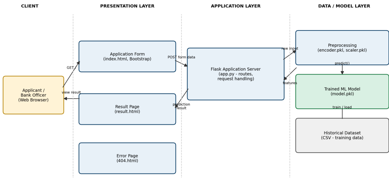
Figure 1: Architecture and data flow of the Credit Card Approval Prediction System, from applicant request through the Flask application, preprocessing pipeline, and trained ML model, back to the result page.
